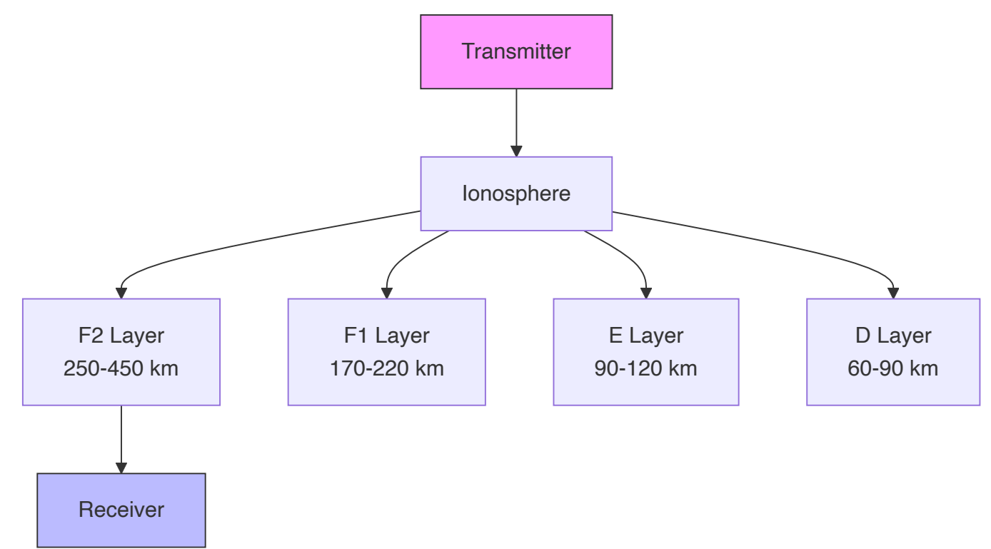
Diagram: Ionospheric Layers and Sky Wave Propagation
