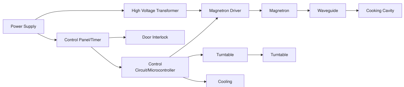
Microwave Oven Block Diagram:
