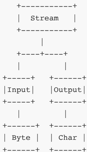
Diagram: Java I/O Hierarchy
